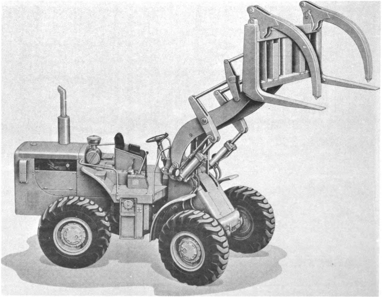
Figure 7-30. Fork and grapple attachment.
